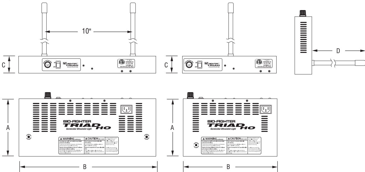
Fig. 3 Dimensions of single and dual lamp Triad HO.
